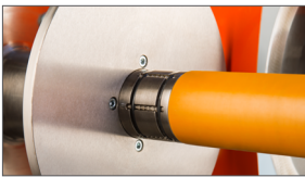
Full pneumatic automatic expansion of the mandrel to block the rolls on shaft
