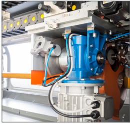
Compact cutting unit positioned at the top for easy cleaning of the working area
